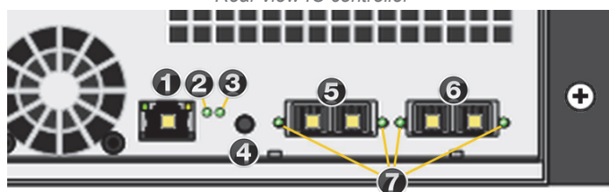
Rear view IO controller
